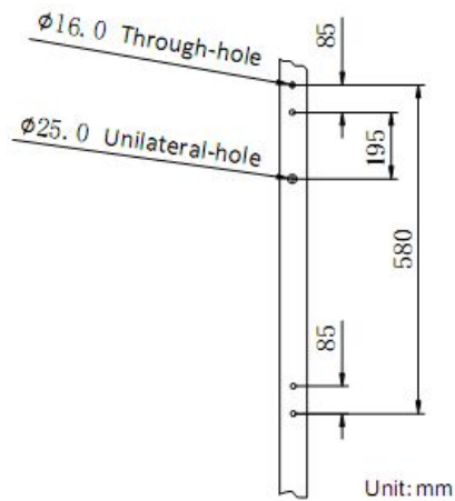
Light pole Installation Holes Chart
